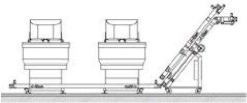
两台MD-W和面机用运输带的配置的例子 Example of configuration — two MD-mixers with transport belt
